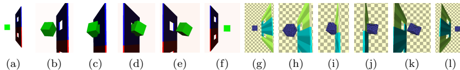
Figure 3.8: 6-dimensional planning: (a-f) Execution of a planned trajectory in the OpenRAVE environment used for planning, (g-l) execution of the same trajectory in the Bullet physics simulator.
