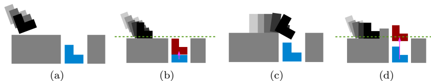
Figure 8.3: Our contact motion controller helps mitigate the effects of contact friction. (a) The robot approaches contact while moving towards the goal in blue. (b) The robot makes contact and becomes stuck on the surface, from which we estimate a plane (green) that locally approximates the surface and adjust the goal by \epsilon_{adjust} shown in magenta to reduce contact force until (c) the robot resumes moving. (d) Alternatively, the robot remains stuck for i iterations until i\epsilon_{adjust} = \epsilon_{adjust}max and the controller terminates.
